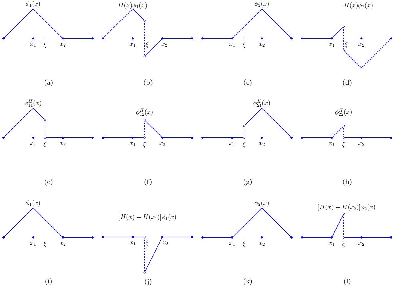
Fig. 3: Basis functions for a discontinuity in one dimension. (a)–(d) X-FEM with generalized Heaviside enrichment; (e)–(h) Approach of Hansbo and Hansbo (2004) ; and (i)–(l) Shifted Heaviside enrichment.
