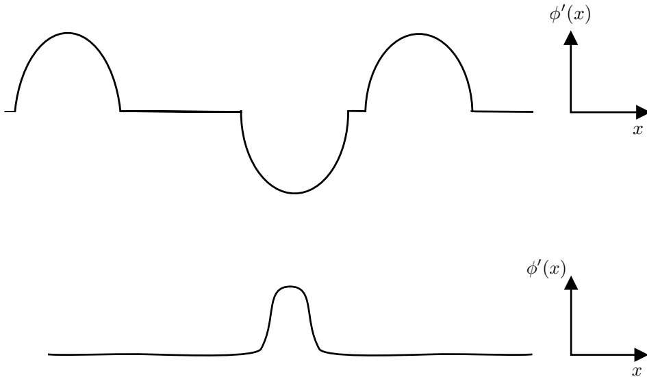
Fig. 4. Top panel: Schematic plot of a generic bounded equilibrium solution of case 3 of Proposition 3.1. Bottom panel: Schematic plot of a solution connecting equilibria of the pendulum equation.
