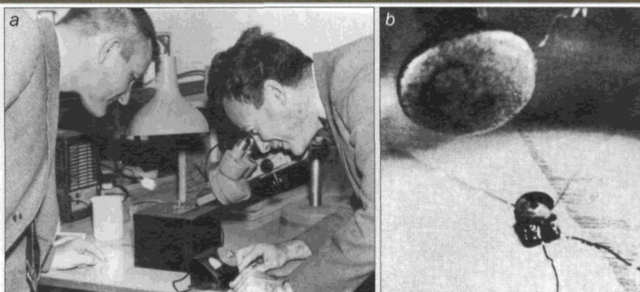
(a) Richard Feynman viewing the micromotor built by William McLellan (left) who won the challenge to build the first motor smaller than 1/64th of an inch. (b) The motor, 3.81 mm wide, photographed under an optical microscope. The huge object above it is the head of a pin.
