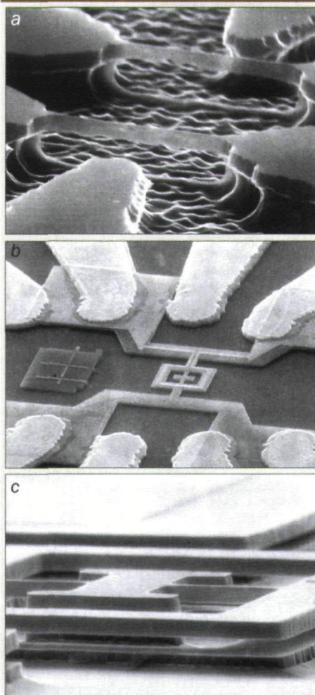
Continued improvements in nanofabrication processes have led to progressively more ideal structures. (a) An early (and rather rough) doubly clamped beam “carved” from a silicon wafer. (b) A compound torsional resonator made from silicon-on-insulator, and (c) a “clean” example made from gallium arsenide that is used to measure minute forces at high frequencies.
