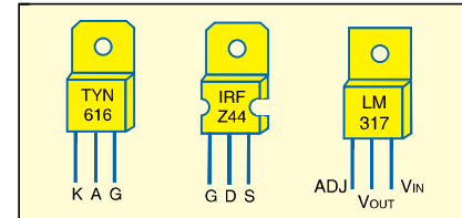
Fig. 3: Pin configurations of TYN616, IRFZ44 and LM317
