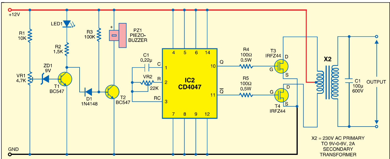
Fig. 2: Simple inverter
