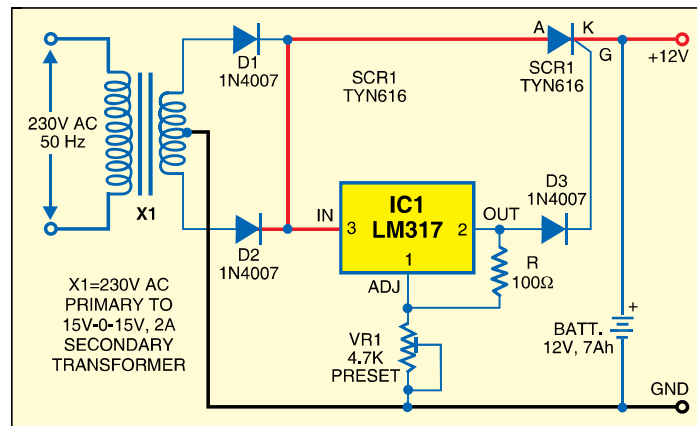
Fig. 1: Battery charger
