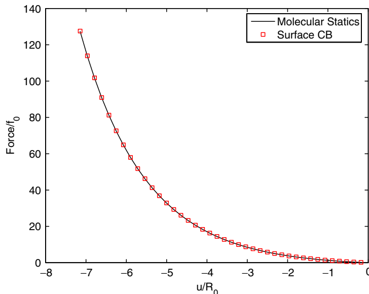
Figure 6. Load versus displacement for full molecular statics and surface Cauchy–Born model for compression of 1D atomic chain after initial relaxation.
