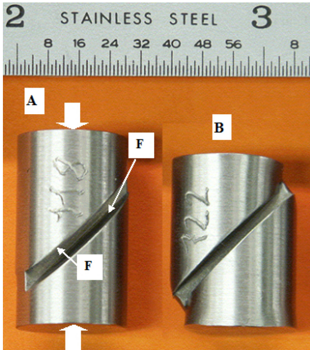
FIG. 1 (color online). A typical shear compression specimen before (A) and after deformation (B). The block arrows show the applied load direction and the thin arrows point to the stress-concentration fillets (F) where ASB's form. Specimens for transmission electron microscopy were taken from this area. Note the shear dominant kinematics in (B).
