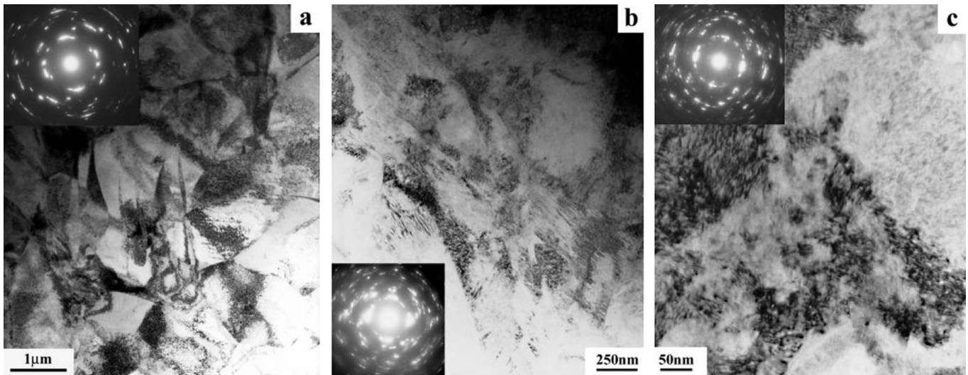
FIG. 4. Dynamically failed specimen—TEM micrographs. (a) Far from the ASB: Dislocation cells and stress-induced martensite. The typical SADP mainly contains misoriented \alpha phase cells. (b) Within the ASB: High dislocation density without any distinct morphology. The SADP shows incomplete rings indicating the presence of very fine recrystallized grains. (c) Higher magnification of (b): The high dislocation density screens the fine grains revealed by the SADP.
