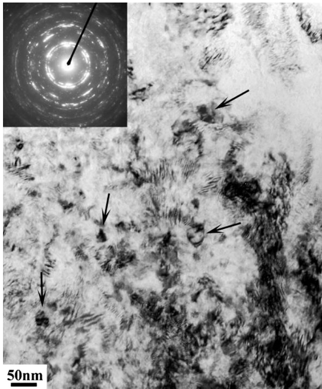
FIG. 5. Interrupted dynamic tests—TEM micrographs in the fillet area. Dynamically recrystallized grains formed in the highly dislocated area are indicated by arrows. The size of the grains ranges from 10–30 nm and they are free of dislocations. The corresponding SADP consists of ring patterns, typical of nanograined polycrystalline materials. Note the similarity of morphologies between this figure and 4(c), namely, high dislocation density and the presence of very fine recrystallized grains.
