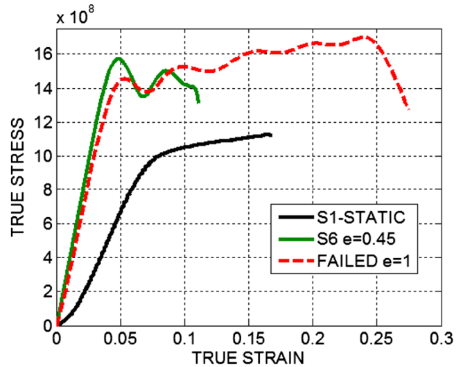
FIG. 2 (color online). True-stress strain curves. S1 was loaded quasistatically up to \epsilon \approx 0.17 and unloaded without failure. “Failed” indicates a specimen that was loaded dynamically until failure by ASB formation. The strain to failure was \epsilon \approx 0.24 , which is used to normalize the strain of S6. The latter was loaded dynamically up to a relative strain of 0.45, and did not fail.
