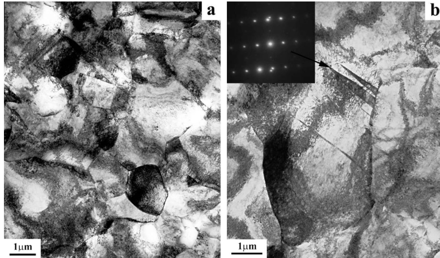
FIG. 3. Quasistatic specimen—TEM micrograph: (a) The typical microstructure consists of dislocation cells. (b) Area showing stress-induced ( \alpha'' ) martensite (arrowed) transformed from the \beta phase, and its corresponding SADP.
