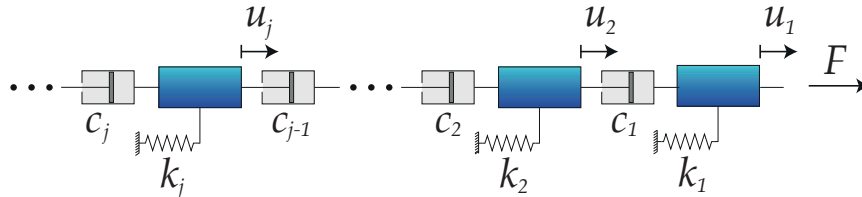
Figure 10. The mechanical hierarchy of the microstructure at the j^{\text{th}} observation scale.
