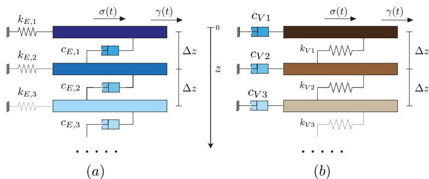
Figure 6. Fractional mechanical model: discrete counterpart of (a) EV and (b) VE materials.
