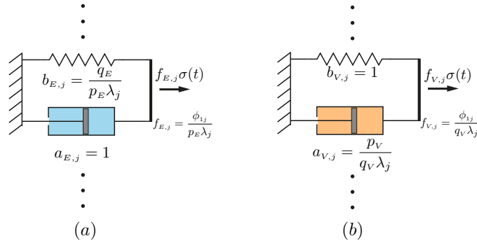
Figure 7. The j^{th} EV (a) and VE (b) Kelvin-Voigt resolution model in modal space.
